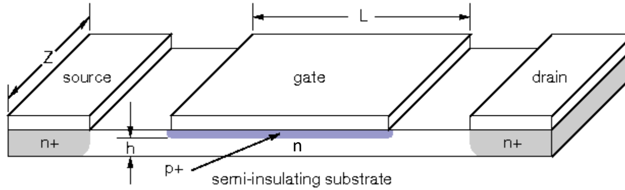
n-channel JFET
