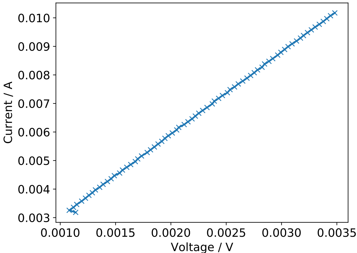
Characteristic IV curve of a silver thin film at 21.174 °C
