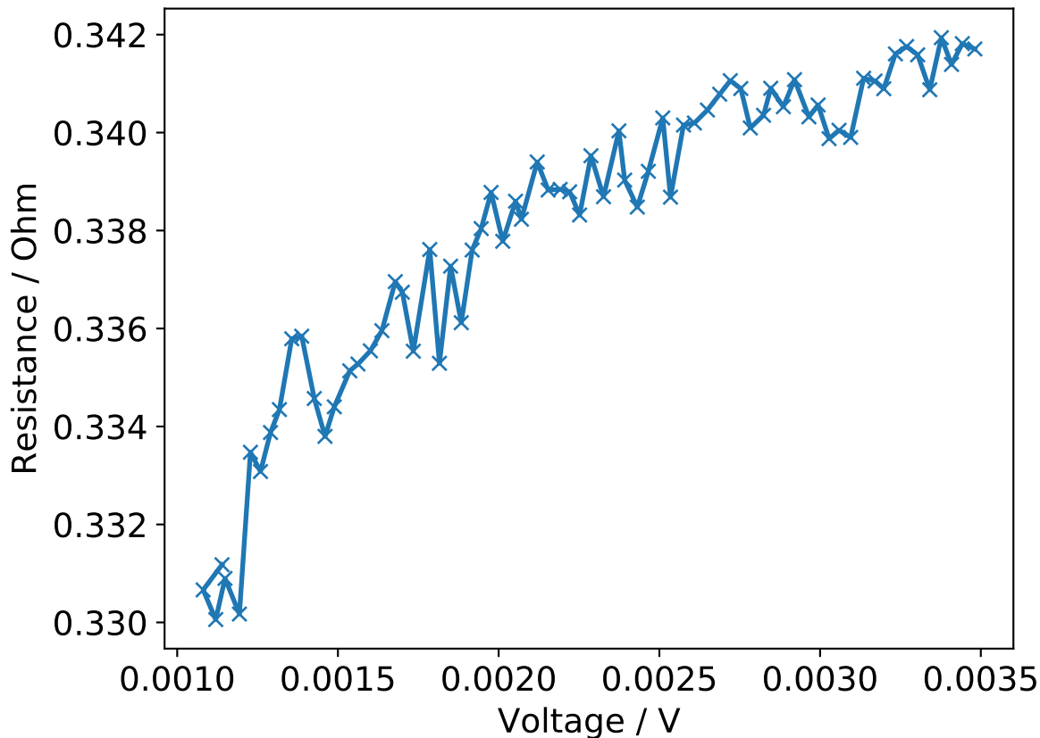
Characteristic RV curve of a silver thin film at 21.174 °C
