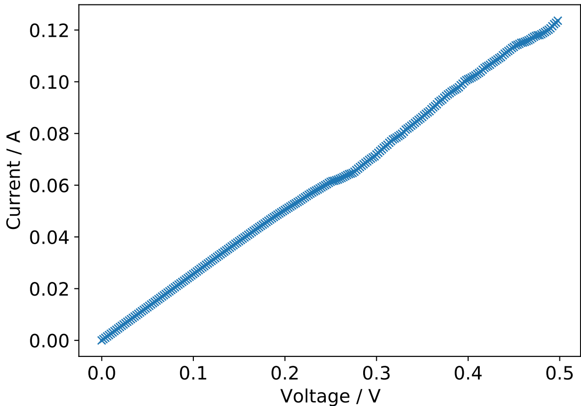
Characteristic curve of a silver film
